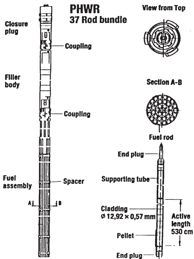
FIG. 46. Fuel assembly for pressure vessel HWR.
