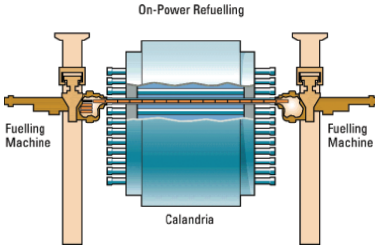
FIG. 9. On-power refuelling.
