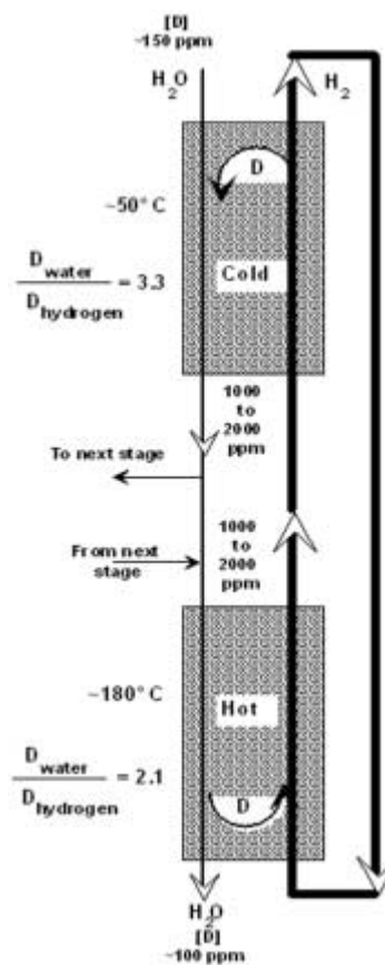
FIG. 78. Schematic diagram of a bithermal process.
