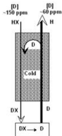
FIG. 77. Schematic diagram of a monothermal process.
