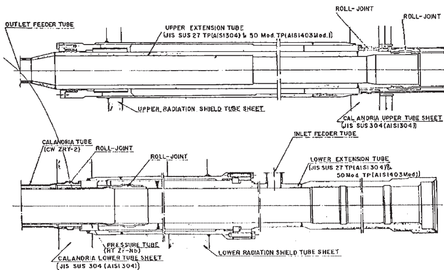
FIG. 71. Fugen fuel channel arrangement.
