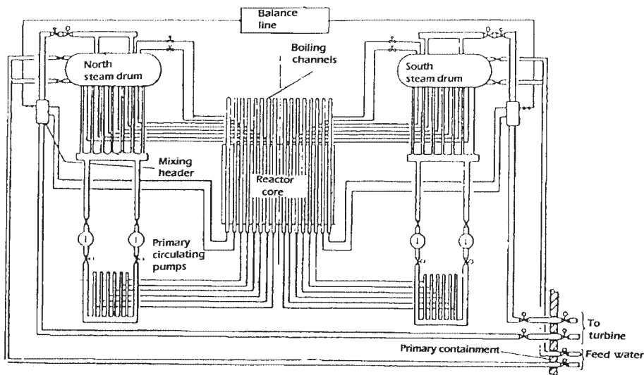
FIG. 26. Primary circuit arrangement for the SGHWR.
