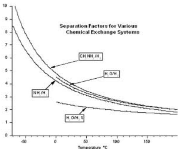
FIG. 79. Separation factors for the main chemical exchange systems as a function of temperature.
